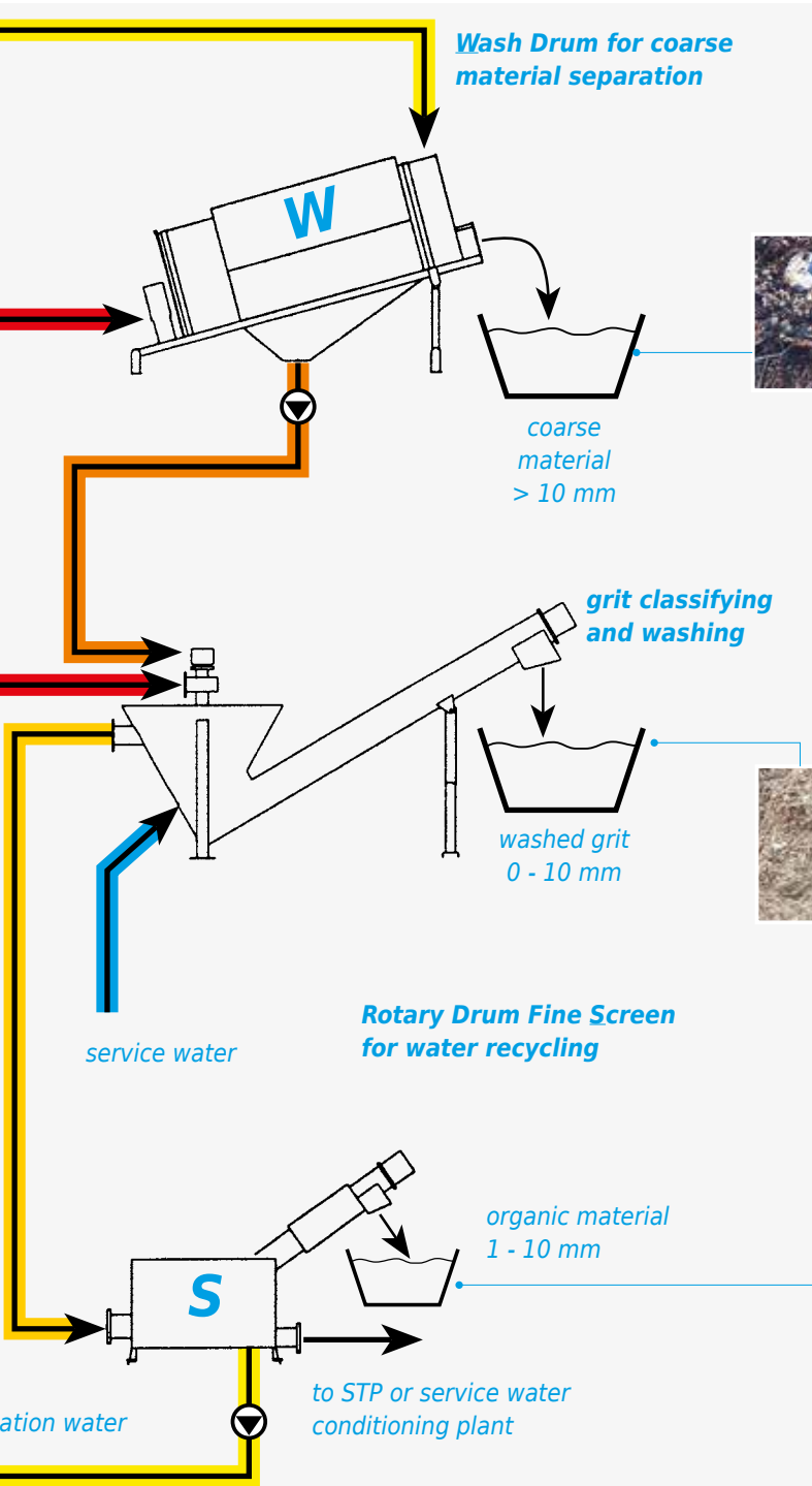
HUBER Wash Drum for washout and separation of all coarse material > 10 mm.
